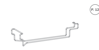
WINE GLASS HOLDER L15" H2.5" W4.5" L37.5cm H6.5cm W11cm Fits Large wide bar shelf Holds up to 6 wine glasses
